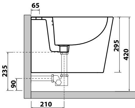
VISTA LATERALE LATERAL VIEW
